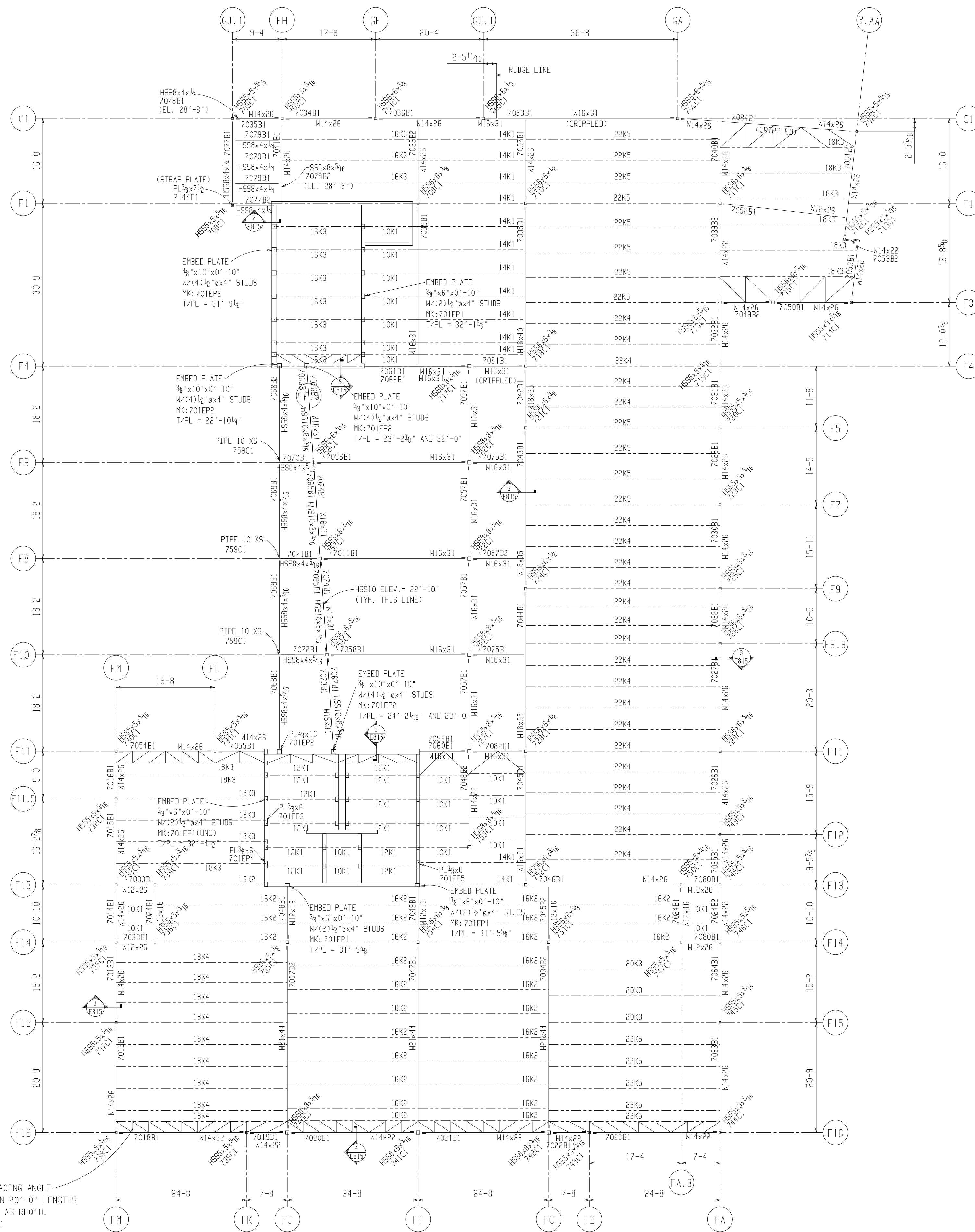
AREA F - ROOF FRAMING PLAN REF 2 E702
