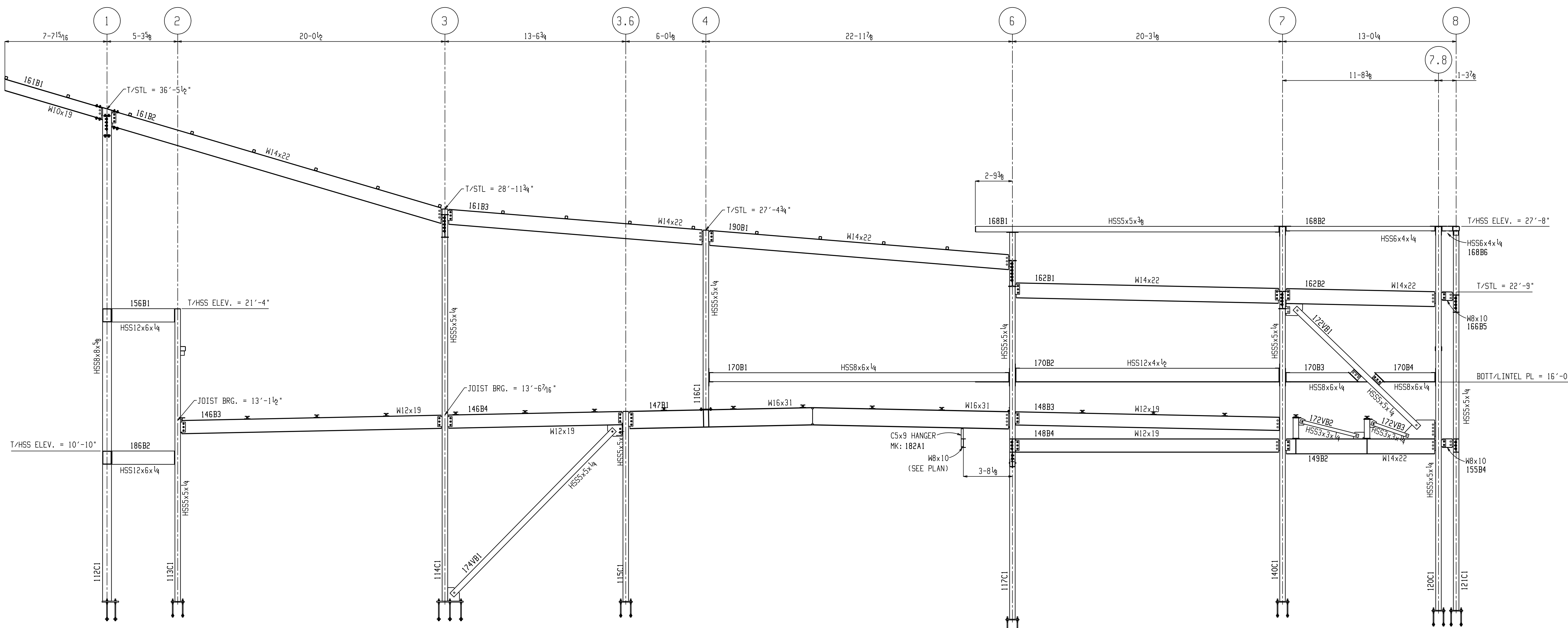
BUILDING ELEVATION 1 E206 ALONG LINE D
