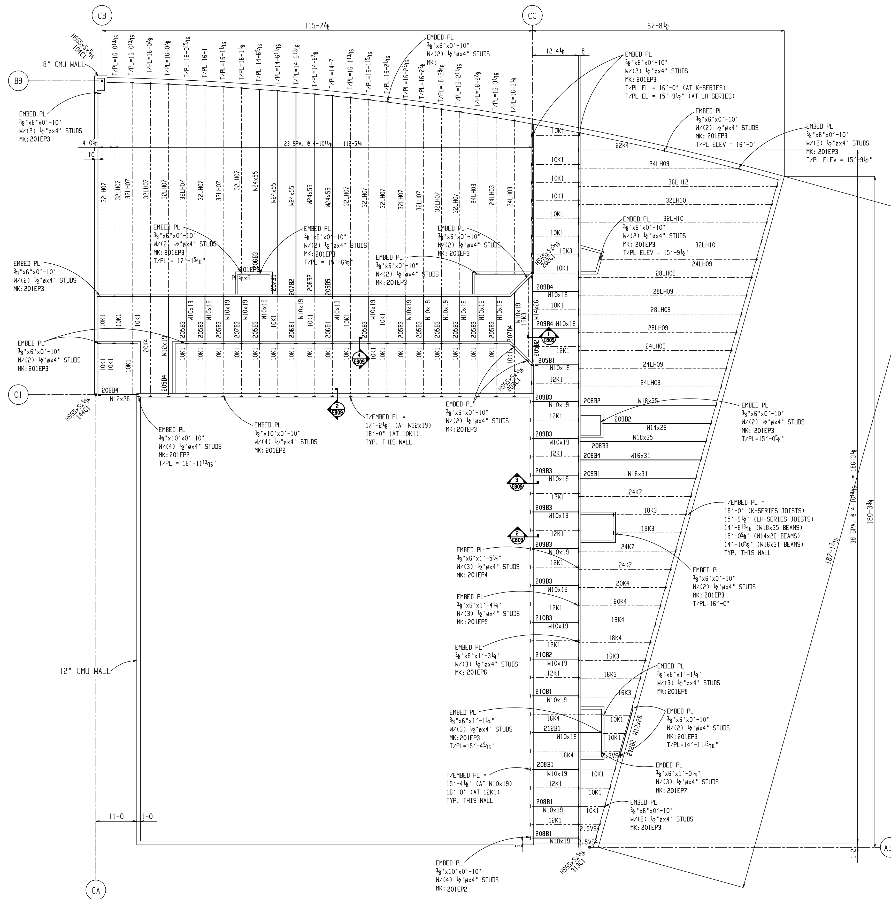
LOW ROOF FRAMIN PLAN ~ AREA C 1 E203
